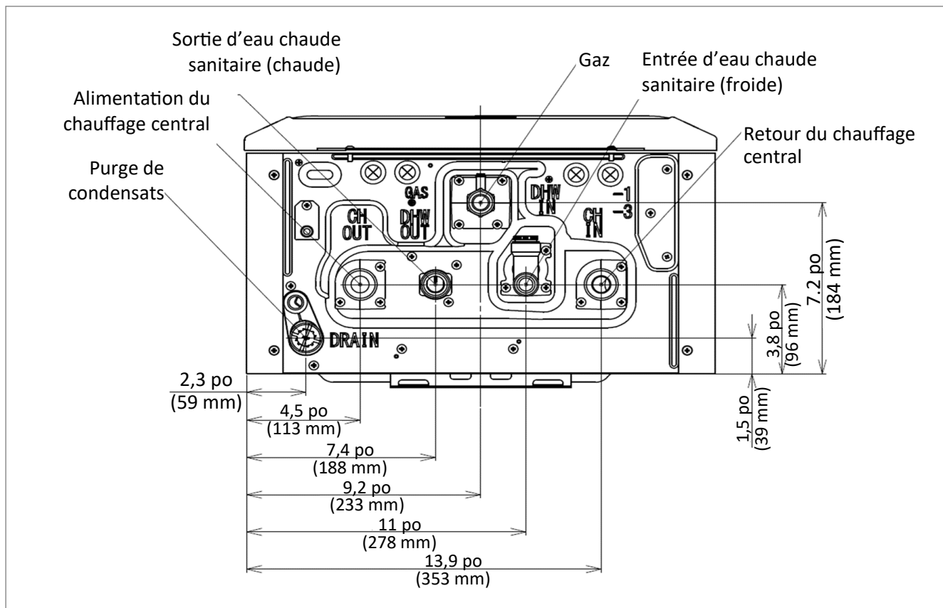
Figure 6: Raccords d'alimentation
